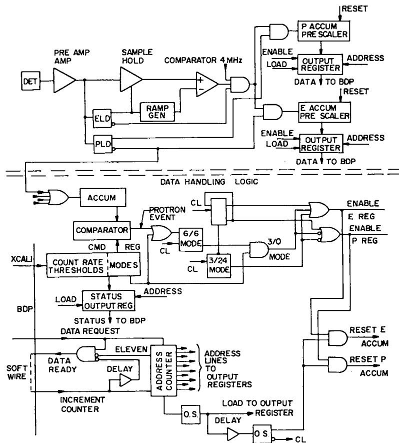
Fig. 9. Block diagram of the BDD electronic circuits.
